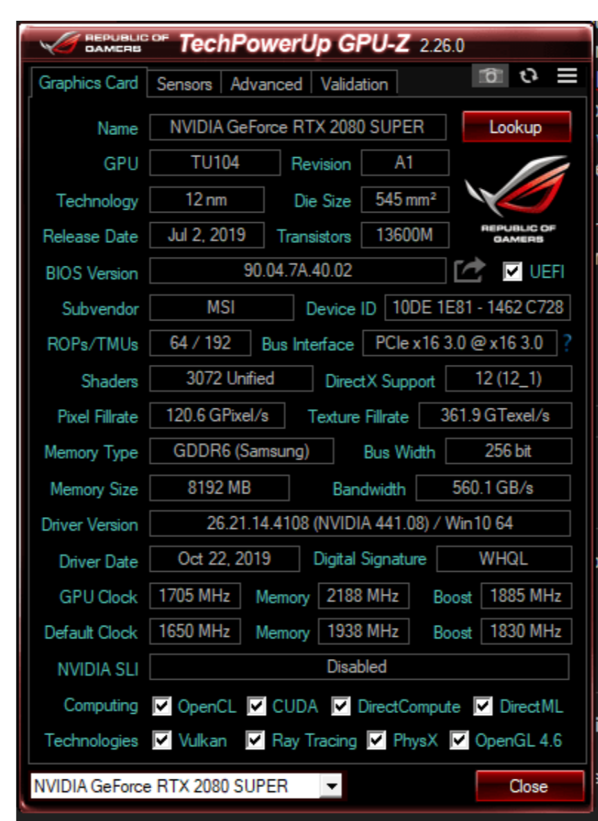
Rtx-2080-gpu-usage-drops
